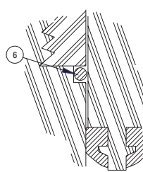
Detail "Y" Enlarged View 1/4" Size Valve
