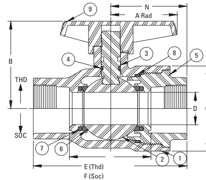
1 1/2" – 2" Conventional Port
