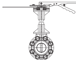
Housed Stem Extension for Butterfly Valves
